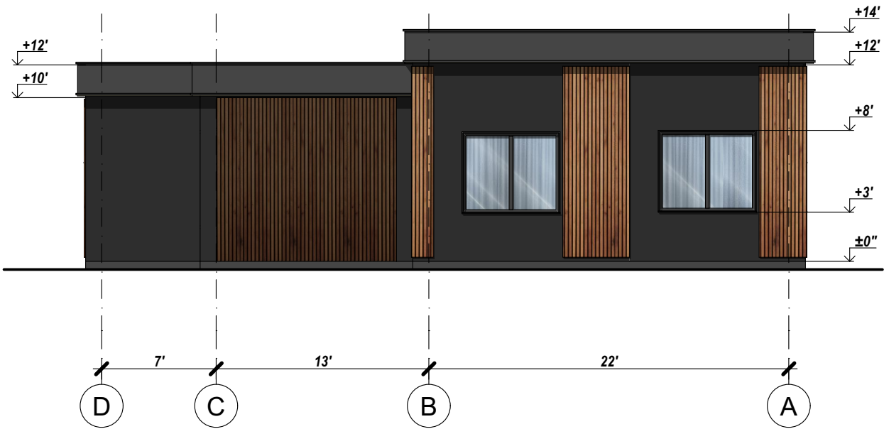
Facade in axes A-D
