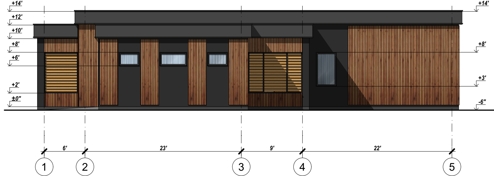
Facade in axes 5-1
