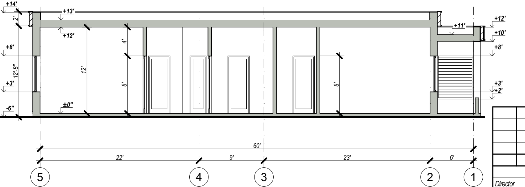
Section 1-1
