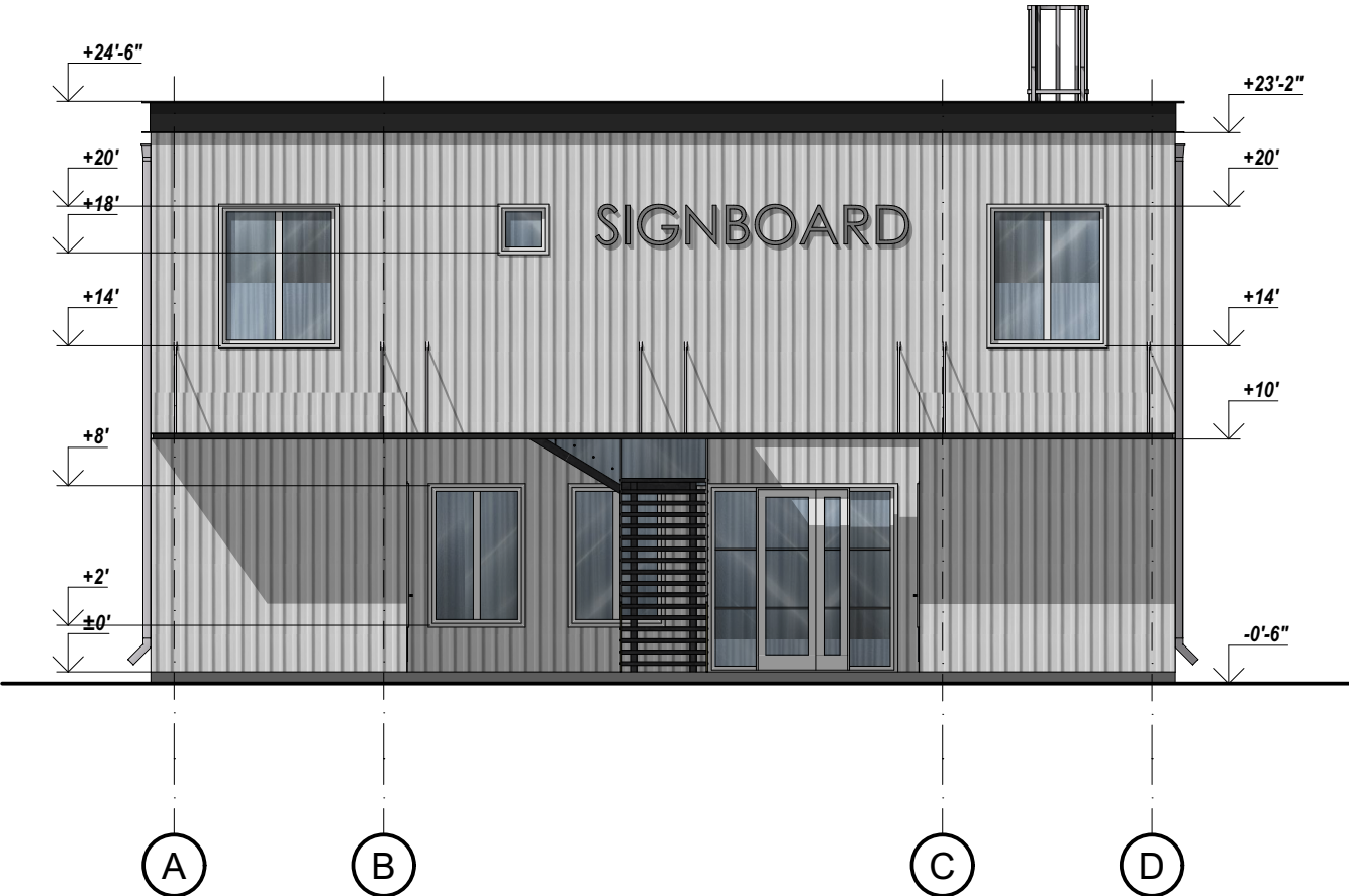
Facade in axes A-D
