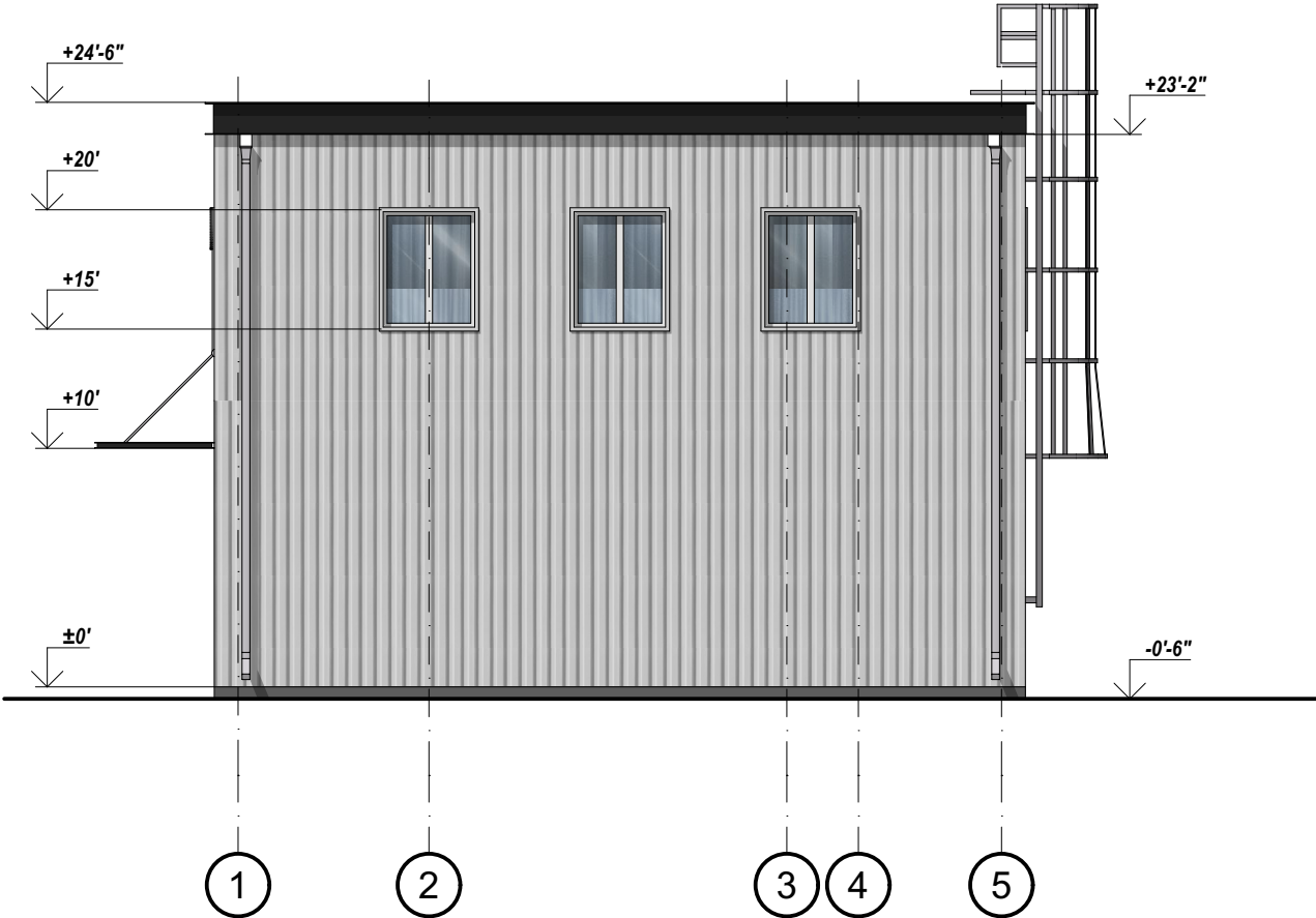
Facade in axes 1-5
