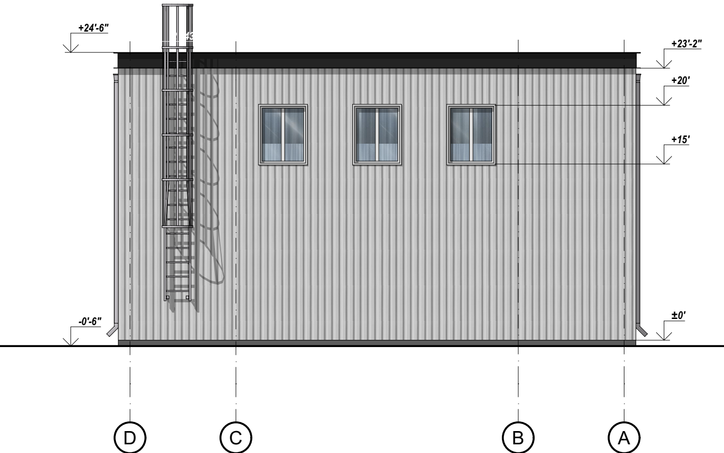
Facade in axes D-A
